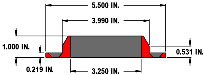
4.0 \varnothing LOCATING RING
